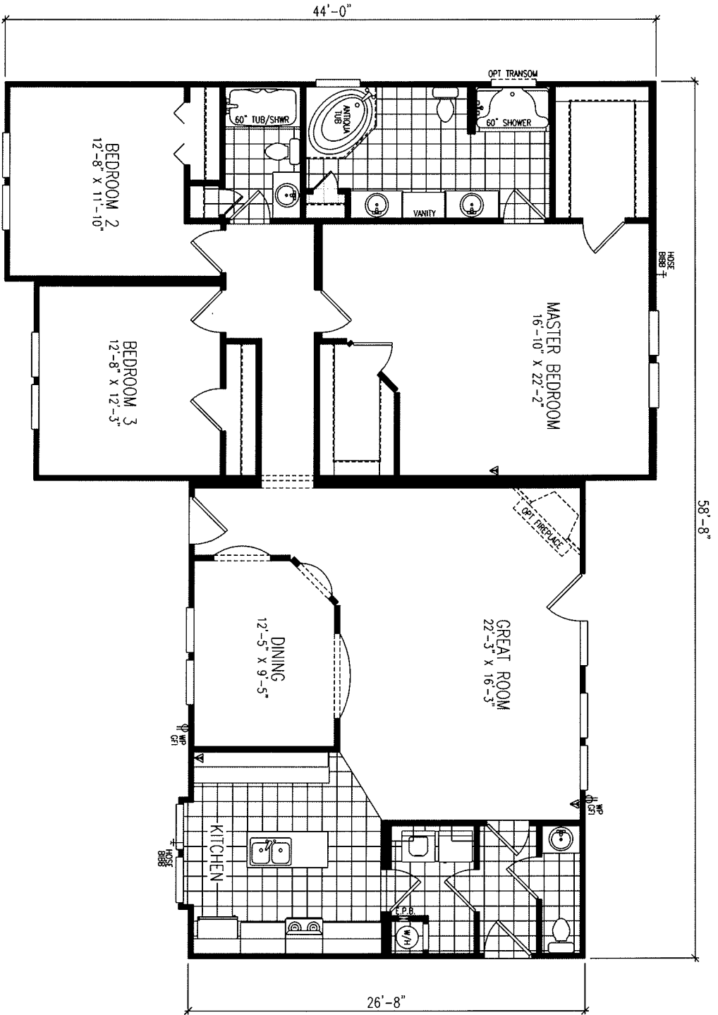
MODEL MD 594-02 3 BR. ~ 2 1/2 BA. 2000 SQ FT HEATED/COOLED
