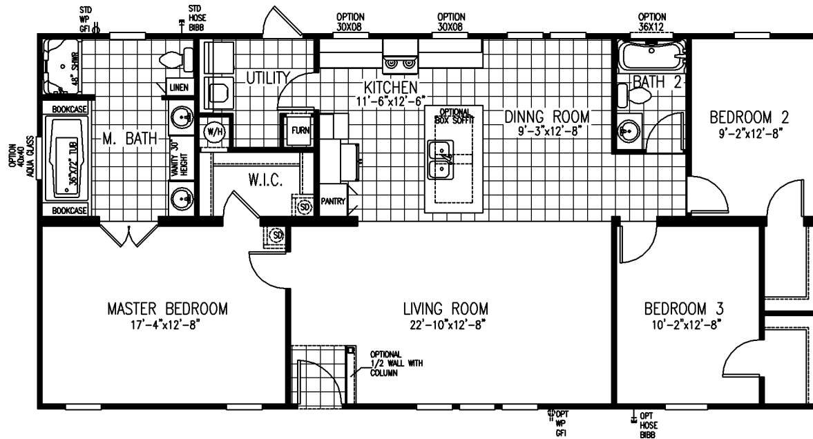
MODEL D603-824 3BR ~ 2BA 28'-0" X 60'-0" ~ 1,493 SQ. FT. ALSO AVAILABLE 32' WIDE
